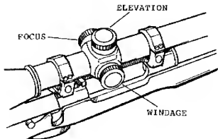
Figure 2-21. Adjustment knobs.
